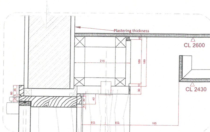
D1 Typical Bulkhead detail
